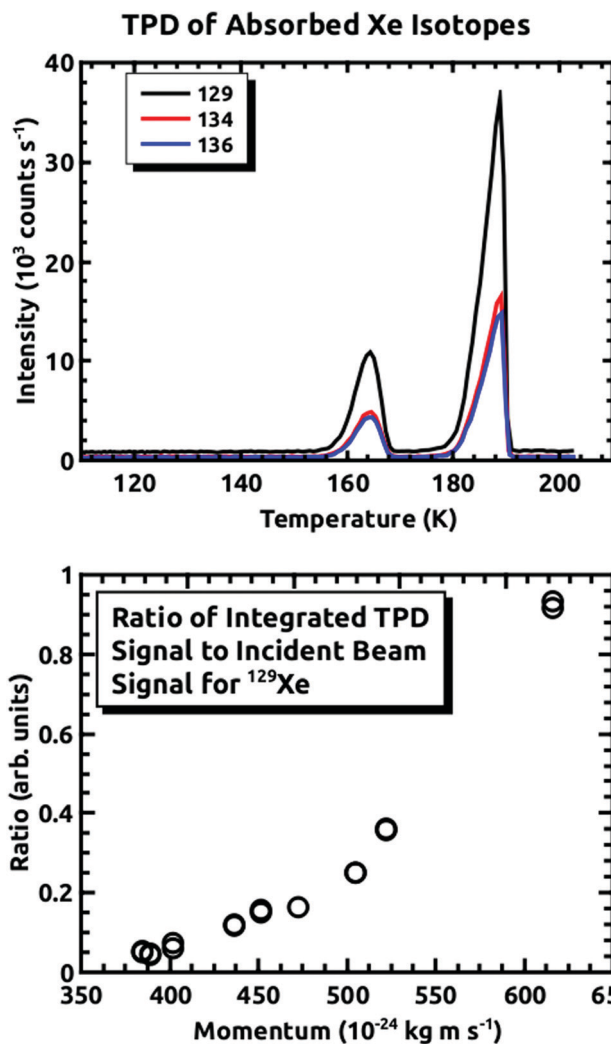
Fig. 3 Top panel: Thermal desorption spectra for the three Xe isotopes taken after a 45 minute exposure of the surface to D 2 O and Xe ( \langle v \rangle = 2.88 \times 10^3 m s -1 ) at \theta_1 = 10^\circ , with a linear ramp rate of 10 K min -1 . Lower panel: relative TPD intensities, normalized by the incident beam intensities, as a function of momentum for 129 Xe.
