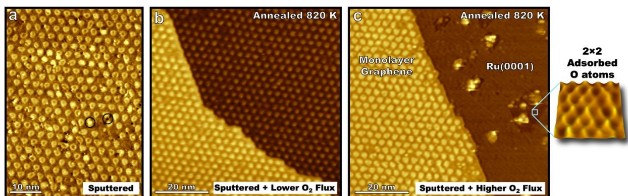
Figure 2. STM images (-1.5 V, -250 pA, 300 K) show the graphene/Ru(0001) interface after Ar + sputtering to induce defects that appear as both bright and dark spots (see encircled examples) at various sites on the moiré lattice and subsequent annealing with O 2 overpressures. Sputtering the surface with 0.5 keV Ar + (60 s, 0.1 \mu A) yielded surface defects seen in (a) at a density of 0.036 defects/nm 2 . After the same sputtering procedure, in separate experiments G/Ru(0001) was exposed to 10 Langmuir of O 2 at 820 K over either 1000 s (b) or 100 s (c). A lower O 2 flux (b, 0.01 Langmuir/s) resulted in largely defect-free G/Ru(0001). A higher O 2 flux (c, 0.1 Langmuir/s) resulted in the erosion of graphene in (c). Note that the graphene edge aligns with the lattice
